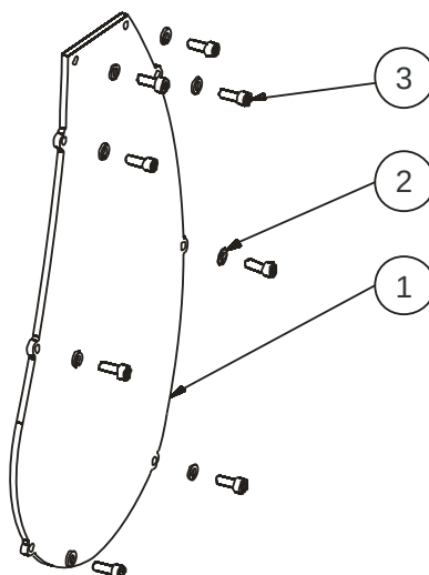
1P02K030 (No. 10) Cover complete
